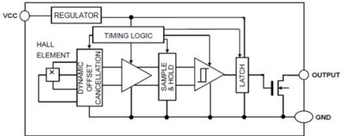
Figure2, Block Diagram of AS1895OD
