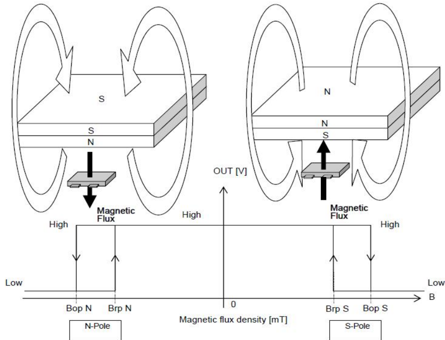
Fig 4, Magnetic Operation Characteristic of AS1895OD
