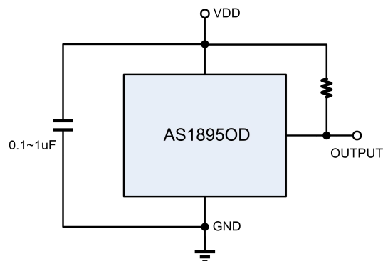
Figure 1, Typical Application Circuit of AS1895OD
